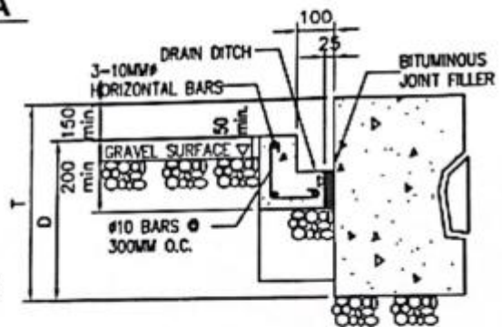
DETAILS "A" SCALE NTS
