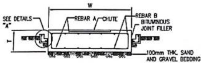
SECTION B
