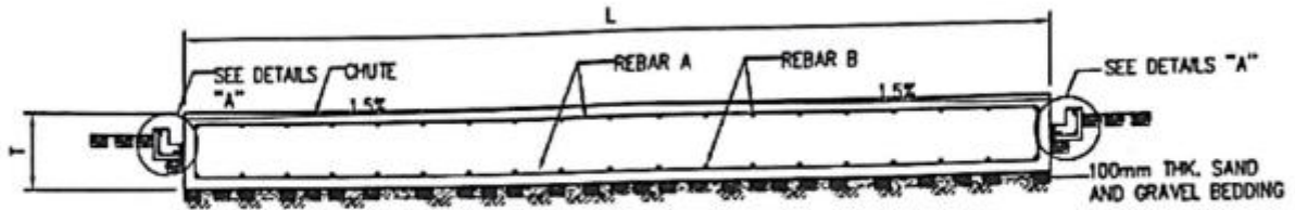
SECTION A
